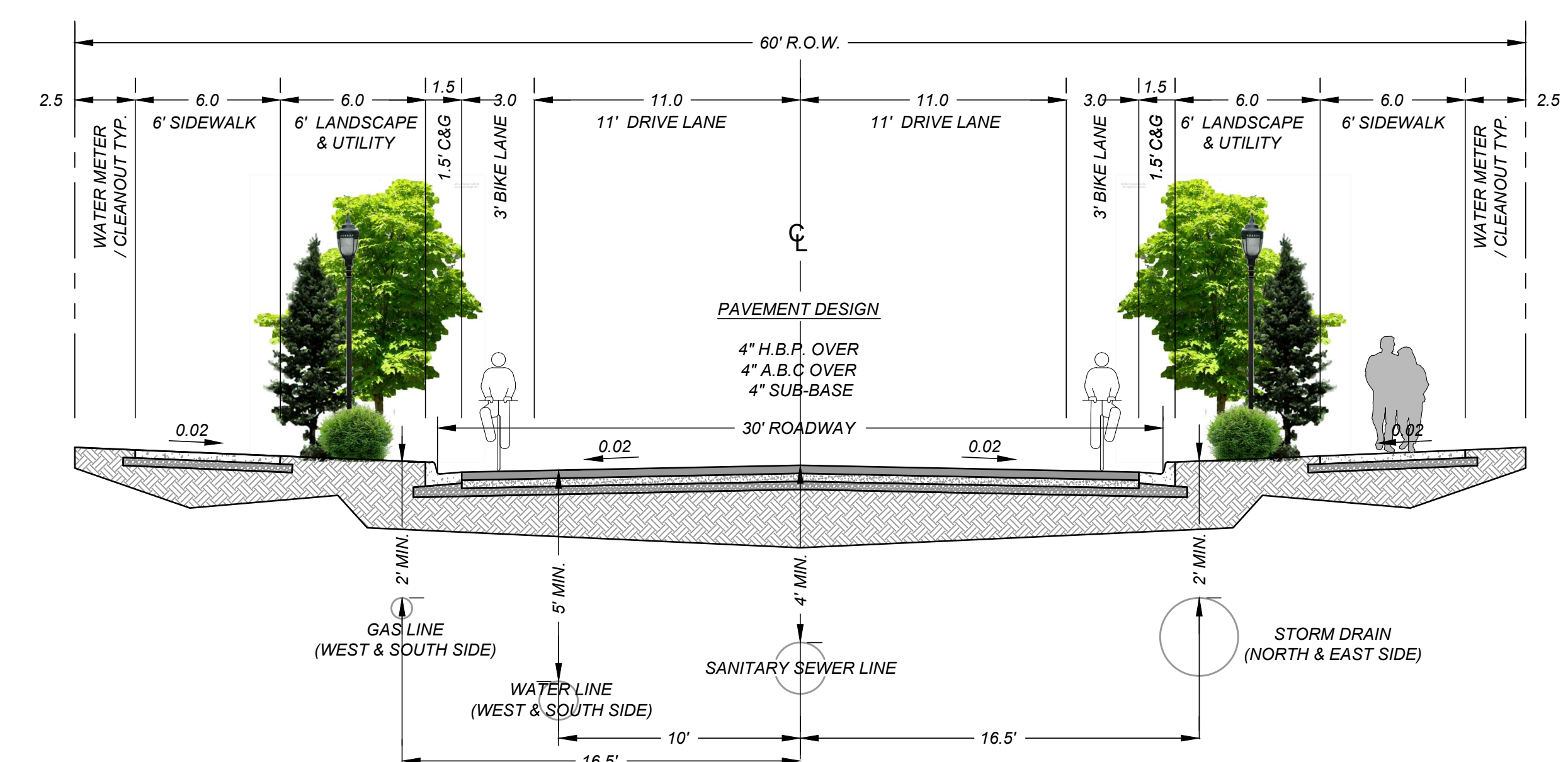
60' R.O.W. MINOR COLLECTOR & UTILITY SECTION SCALE: 1" = 5' NOTES: 1. NORMAL CROWN OF 0.02' PER FOOT UNLESS OTHERWISE DIRECTED BY DIRECTOR OF ENGINEERING. 2. PAVEMENT DESIGN SHALL BE AS SHOWN OR AS CALCULATED ACCORDING TO SPECIFICATIONS, WHICHEVER IS GREATER. 3. REVIEW QUALIFYING CRITERIA AND CROSS SECTIONS FOR "COLLECTOR STREETS".
